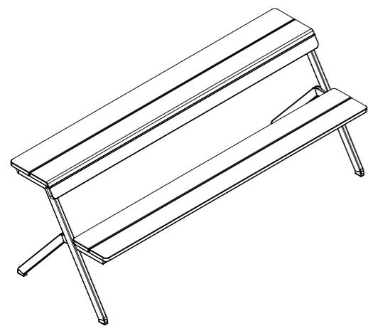
ISOMETRIC
